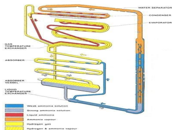
Fig 2 . Electrolux Refrigeration system
